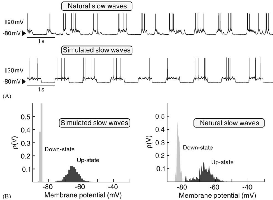
Fig. 3. Model of synaptic bombardment during slow-wave oscillations. (A) For the down-state ( R_{in} = 38 \text{ M}\Omega ), none of the excitatory neurons fires, whereas the release rate at GABAergic synapses was \nu_{GABA} = 0.67 \text{ Hz} ( g_i = 11.85 \text{ nS} ). For upstate, g_i decreased by about 8 \text{ nS} , corresponding to \nu_{GABA} = 0.226 \text{ Hz} , whereas g_e increases by about 6 \text{ nS} , corresponding input frequency \nu_{AMPA} between 0.3 and 0.4 \text{ Hz} . \sigma_i increases by 3\text{--}4 \text{ nS} during the transition to the up-state (corresponding to c_{GABA} = 0.8 ), whereas \sigma_e increases by 2 \text{ nS} (corresponding to c_{AMPA} = 0.4 ). The periods of slow wave were 1 \text{ s} . The slopes of changes in the mean and variance of synaptic conductances were fitted to experimental data. (B) V_m distribution for up- and down-state. The mean membrane potential was -64.80 and -84.90 \text{ mV} , respectively, in accordance with experimental data.
