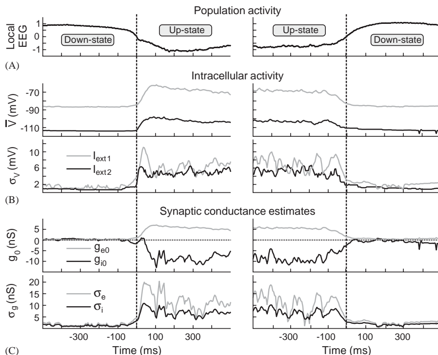
Fig. 1. Characterization of intracellular activity during slow-wave oscillations in vivo. (A) The population activity (local EEG) is used to precisely align individual intracellular recordings (dashed lines) corresponding to the start (left) and end (right) of the up-states characterizing slow-wave oscillations. (B) Gaussian approximations of the membrane potential distributions yield the mean \bar{V} and standard deviation \sigma_V as a function of time during slow-wave oscillations. Corresponding values for \bar{V} and \sigma_V at two different currents ( I_{\text{ext}1} = 0.014 nA, I_{\text{ext}2} = -0.652 nA) are shown. (C) With the characterization of the subthreshold membrane potential time course describing intracellular activity during slow waves, the mean g_{e0} , g_{i0} and standard deviation \sigma_e , \sigma_i of excitatory and inhibitory conductances can be estimated as a function of time.
