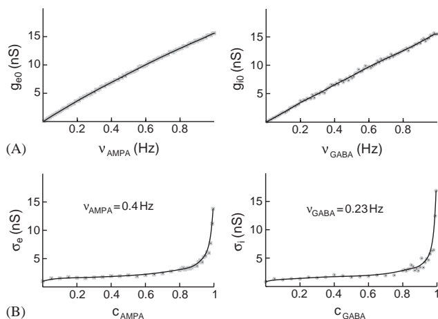
Fig. 2. Computing the correspondence between release parameters and global conductance properties. (A) Relation between mean conductance ( g_{e0} or g_{i0} ) and mean rate of release ( v_{\text{AMPA}} or v_{\text{GABA}} ) at excitatory (left, gray square) and inhibitory (right, gray circle) synapses. (B) Relation between conductance variance ( \sigma_e or \sigma_i ) and the temporal correlation ( c_{\text{AMPA}} or c_{\text{GABA}} ) between excitatory (left, gray square) and inhibitory (right, gray circle) synapses. The mean and variance of conductances were estimated by a somatic voltage-clamp (at 0 and -80 mV, to estimate inhibition and excitation, respectively).
